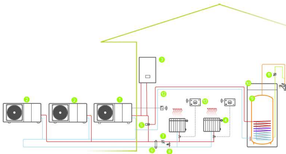
Hybrid single-zone system in cascade:
