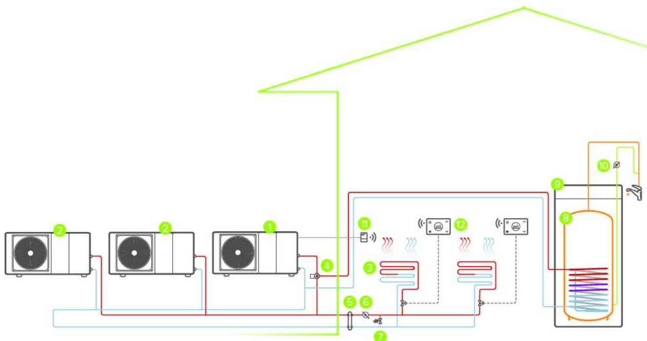
Full electric single-zone system in cascade:
