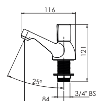
Bath Tap Pair UNEXTPBTH
