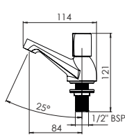
Basin Tap Pair UNEXTPBAS
