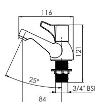
Bath Tap Pair with Lever UNEXTPBTHLE
