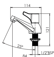
Basin Tap Pair with Lever UNEXTPBASLE
