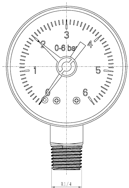
EV-G614SC Gauge 6 Bar 1/4" Side Connection
